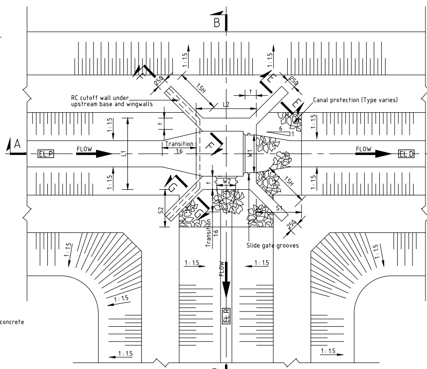
PLAN 1:50 (AT A1) TYPE 1
