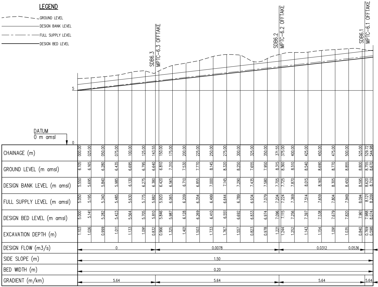
MPSC-6 PROFILE SCALE: Hor 1:2000, Ver 1:100
