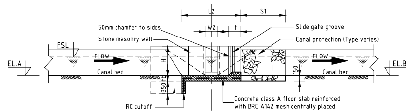
SECTION C-C 1:50 (AT A1)
