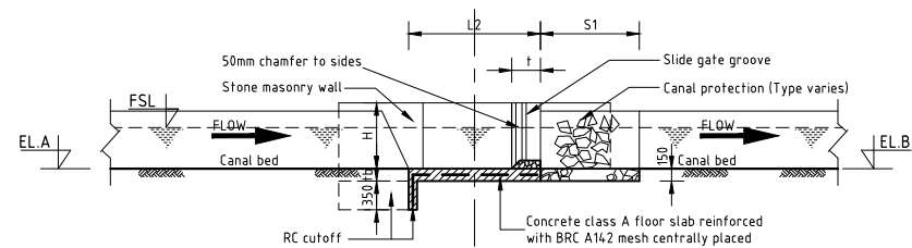
SECTION A-A 1:50 (AT A1)
