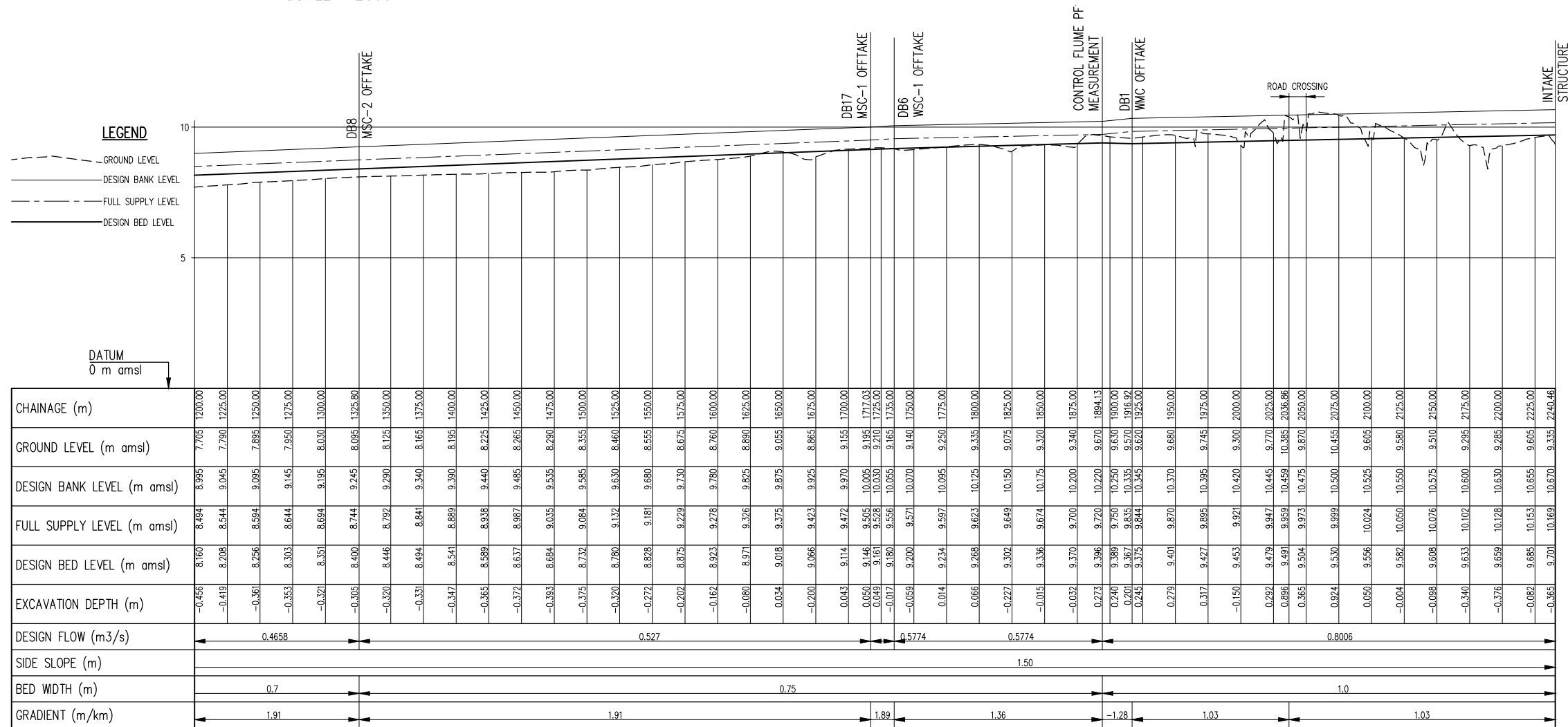
MMC / WMCC PROFILE SCALE: Hor 1:2000, Ver 1:100
