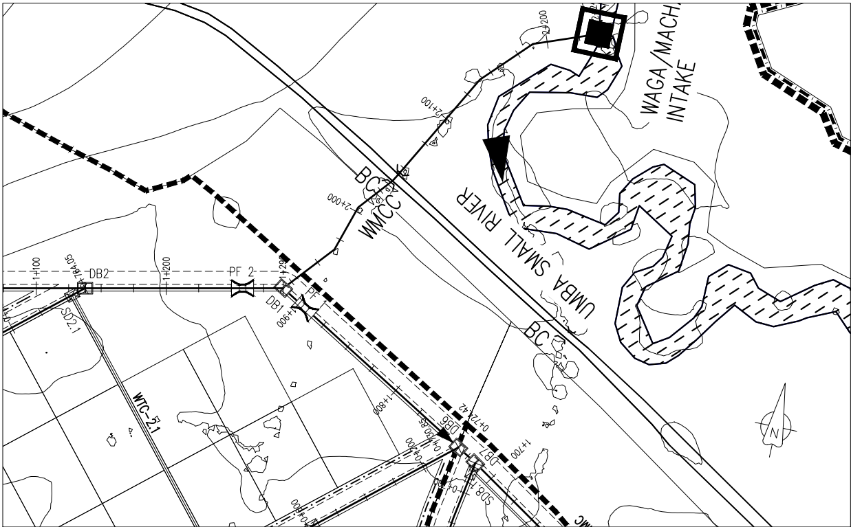
WMC PLAN SCALE 1:2000
