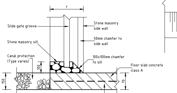
DETAIL 'A' 1:10 (AT A1)
