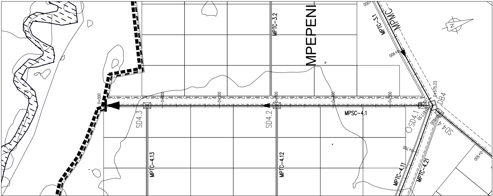
MPSC-4.1 PLAN SCALE 1:2000
