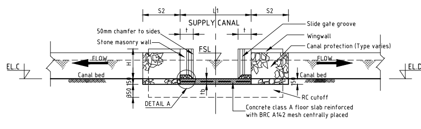
SECTION D-D 1:50 (AT A1)
