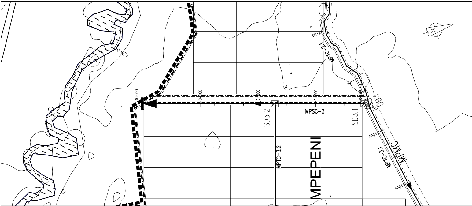
MPSC-3 PLAN SCALE 1:2000
