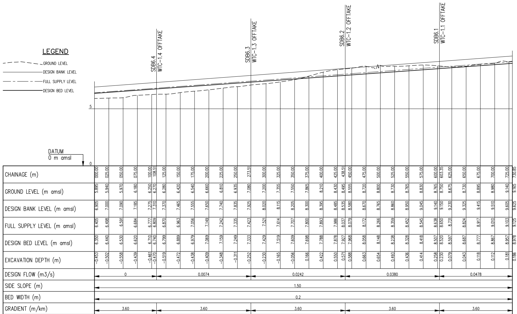
WSC-1 PROFILE SCALE: Hor 1:2000, Ver 1:100
