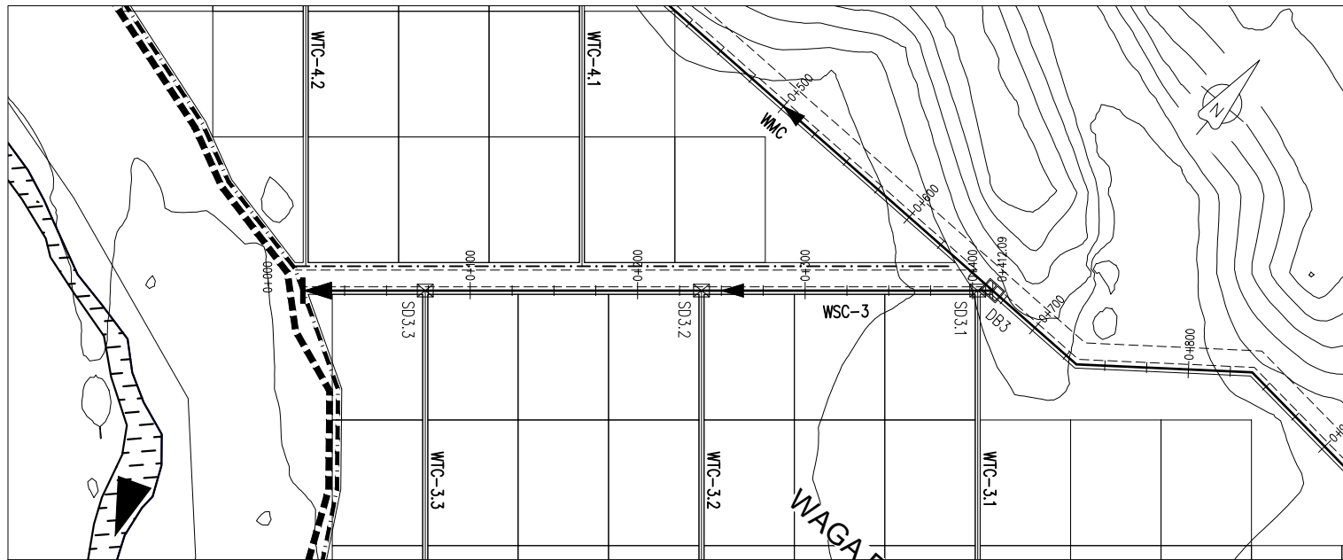
WSC-3 PLAN SCALE 1:2000
