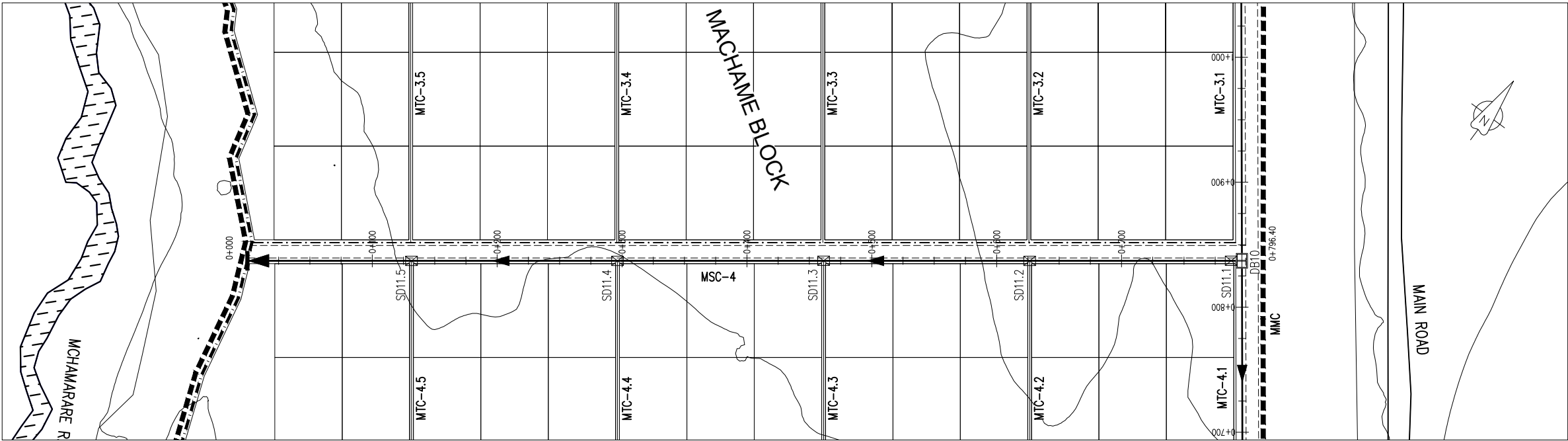
MSC-4 PLAN SCALE 1:2000
