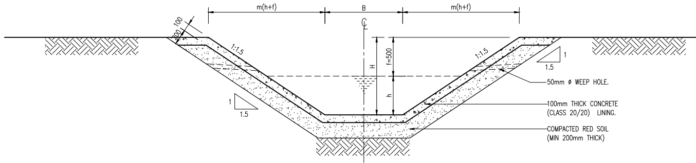
CONCRETE LINED CANAL CROSS SECTION SCALE 1:25
