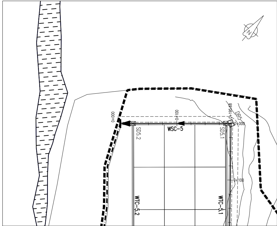
WSC-5 PROFILE PLAN SCALE 1:2000
