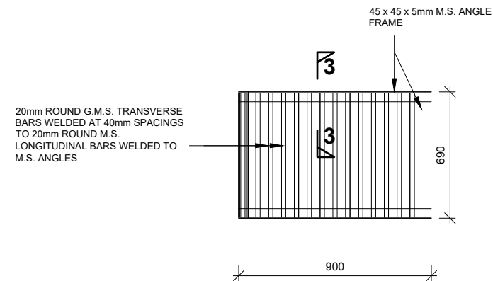
GMS GRATING COVER OVER FINE SCREEN ACCESS OPENING PLAN NTS
