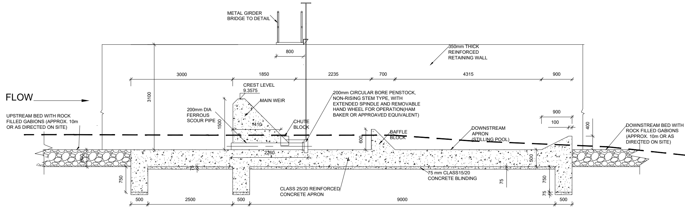
SECTION B-B SECTION THROUGH THE MAIN WEIR
