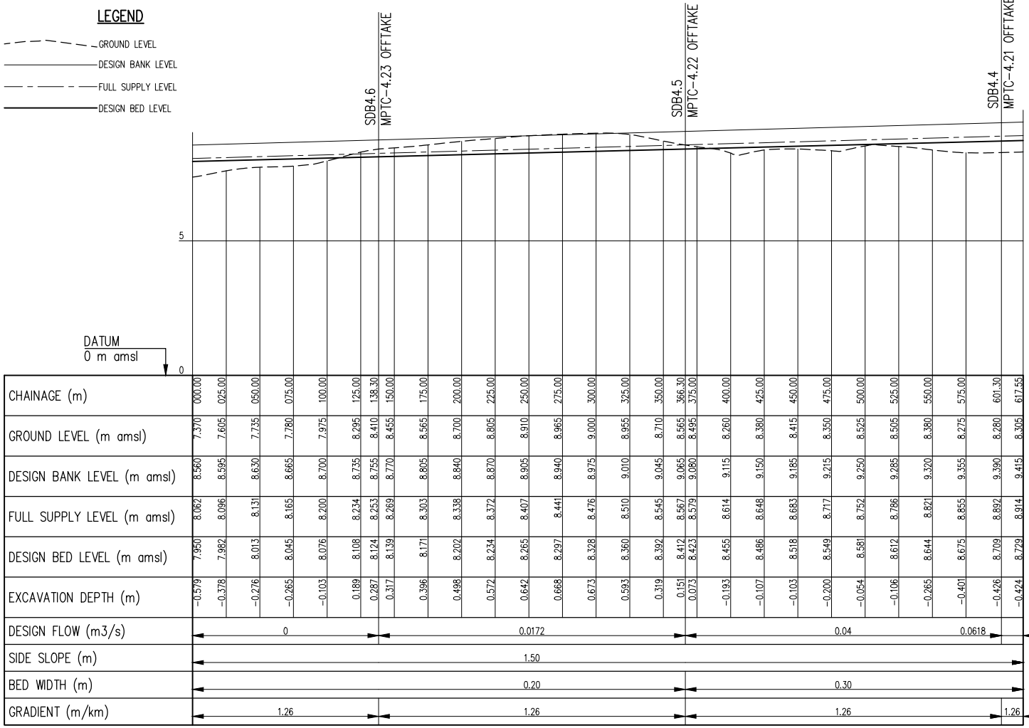
MPSC-4.2 PROFILE SCALE: Hor 1:2000, Ver 1:100
