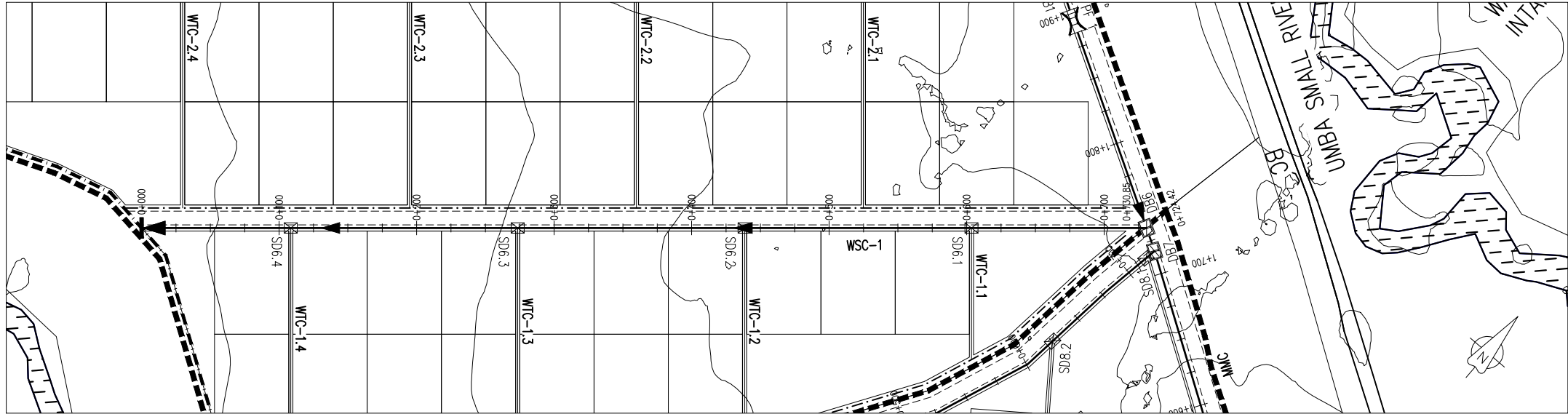
WSC-1 PLAN SCALE 1:2000
