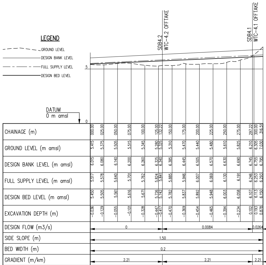
WSC-4 PROFILE SCALE: Hor 1:2000, Ver 1:100
