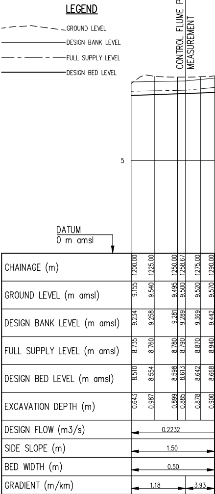
WMC PROFILE SCALE: Hor 1:2000, Ver 1:100
