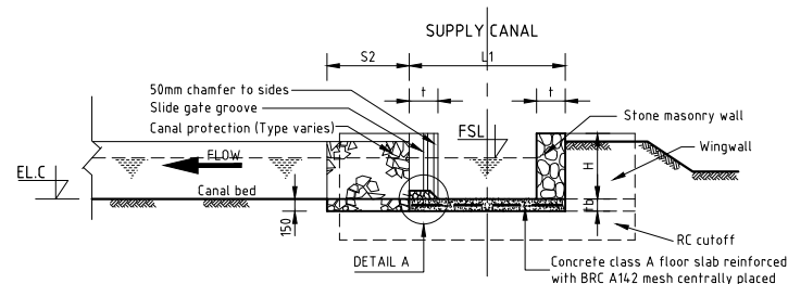
SECTION B-B 1:50 (AT A1)
