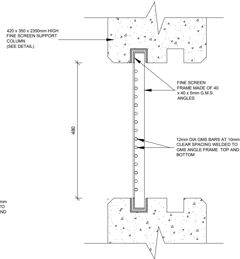
FINE SCREEN AND SUPPORT COLUMN SECTIONAL PLAN NTS
