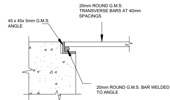
SECTION 3-3 (NTS)
