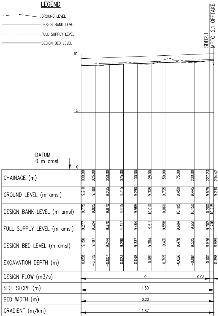
MPSC-2 PROFILE SCALE: Hor 1:2000, Ver 1:100
