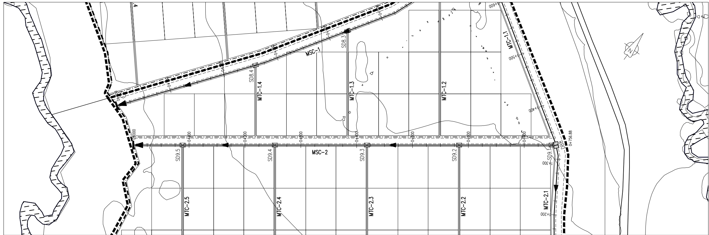
MSC-2 PLAN SCALE 1:2000
