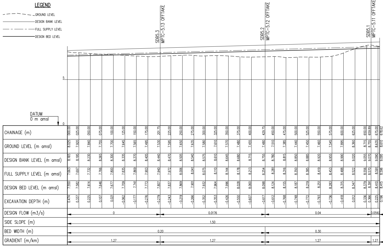
MPSC-5.1 PROFILE SCALE: Hor 1:2000, Ver 1:100
