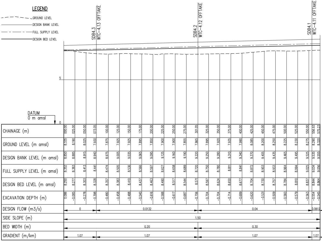
MPSC-4.1 PROFILE SCALE: Hor 1:2000, Ver 1:100
