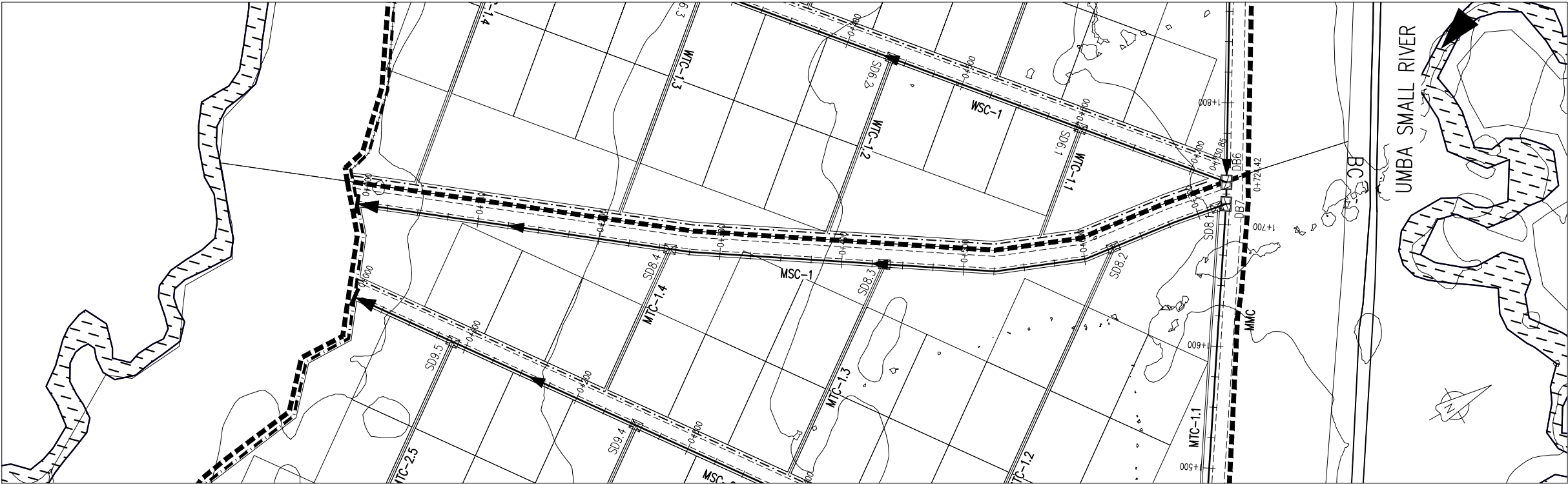
MSC-1 PLAN SCALE 1:2000
