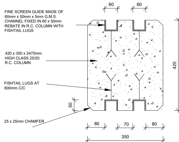
FINE SCREEN SUPPORT COLUMN DETAIL PLAN SCALE 1:10
