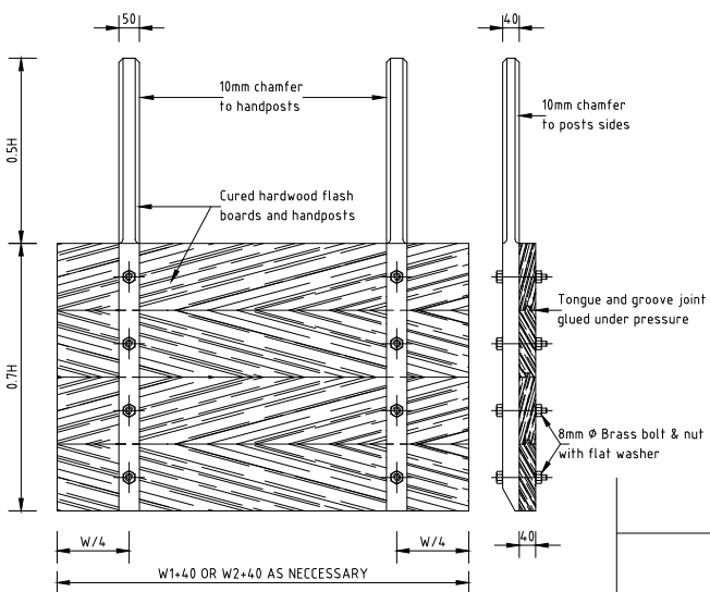
TYPICAL STOPLOG DETAILS 1:10 (AT A1)
