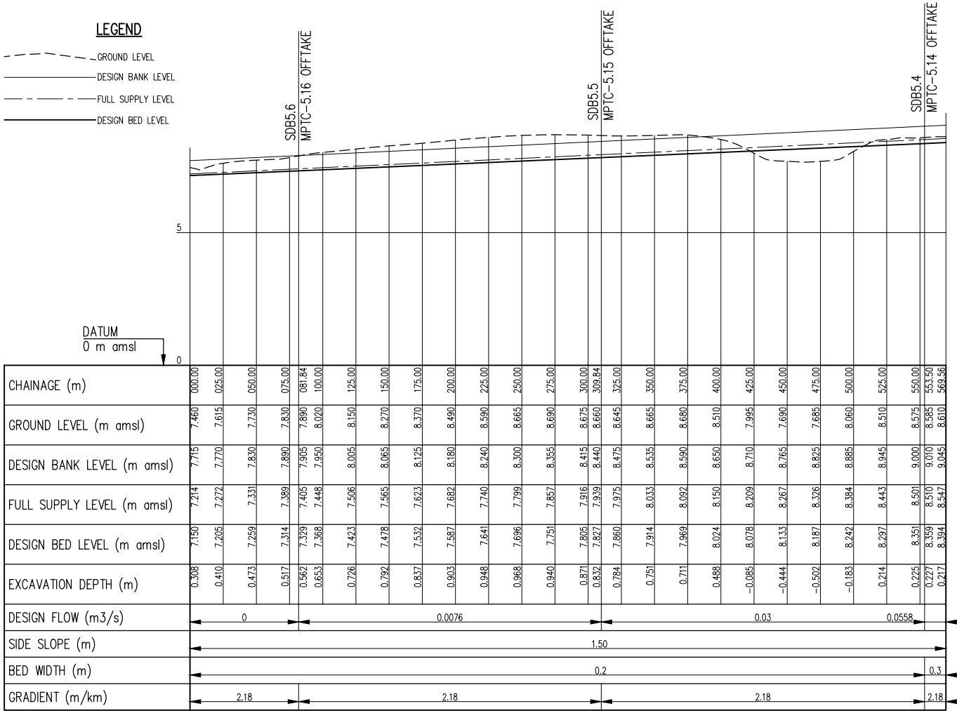
MPSC-5.2 PROFILE SCALE: Hor 1:2000, Ver 1:100
