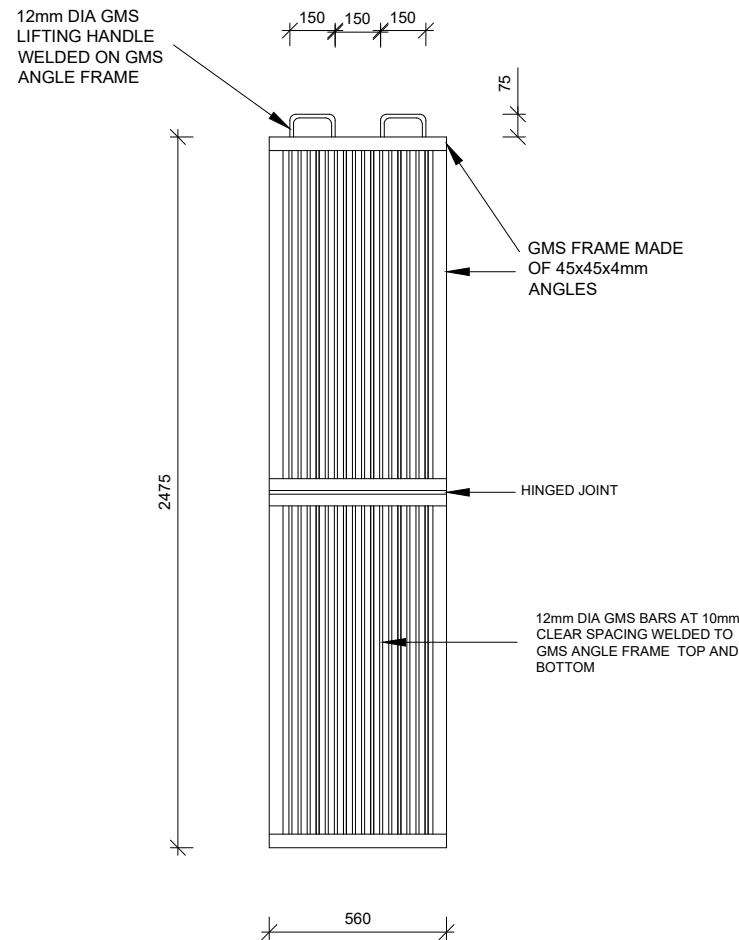
FINE SCREEN ELEVATION SCALE 1:25
