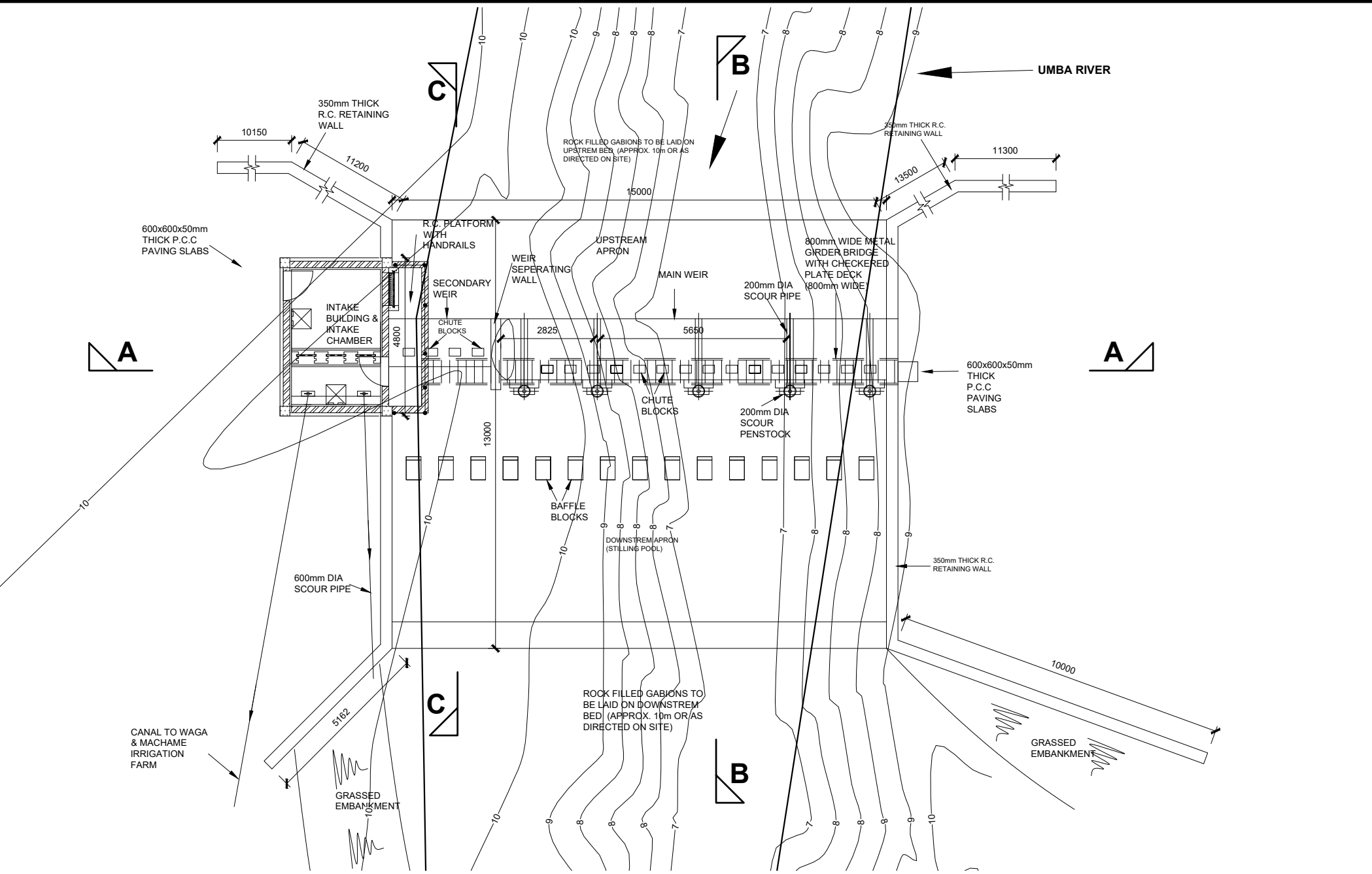
INTAKE WEIR, INTAKE CHAMBER & INTAKE BUILDING PLAN
