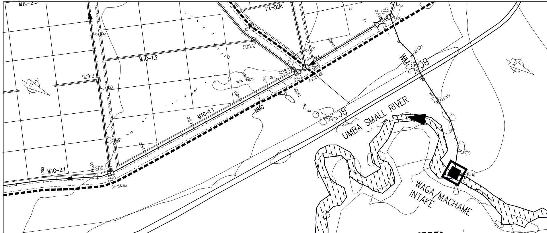
MMC / WMCC PLAN SCALE 1: 2000
