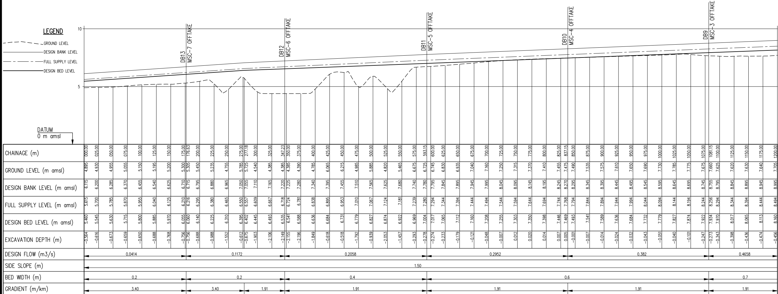
MMC / WMCC PROFILE SCALE: Hor 1:2000, Ver 1:100
