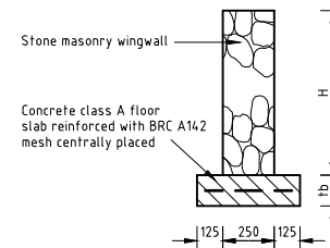
SECTION E-E 1:20 (AT A1)
