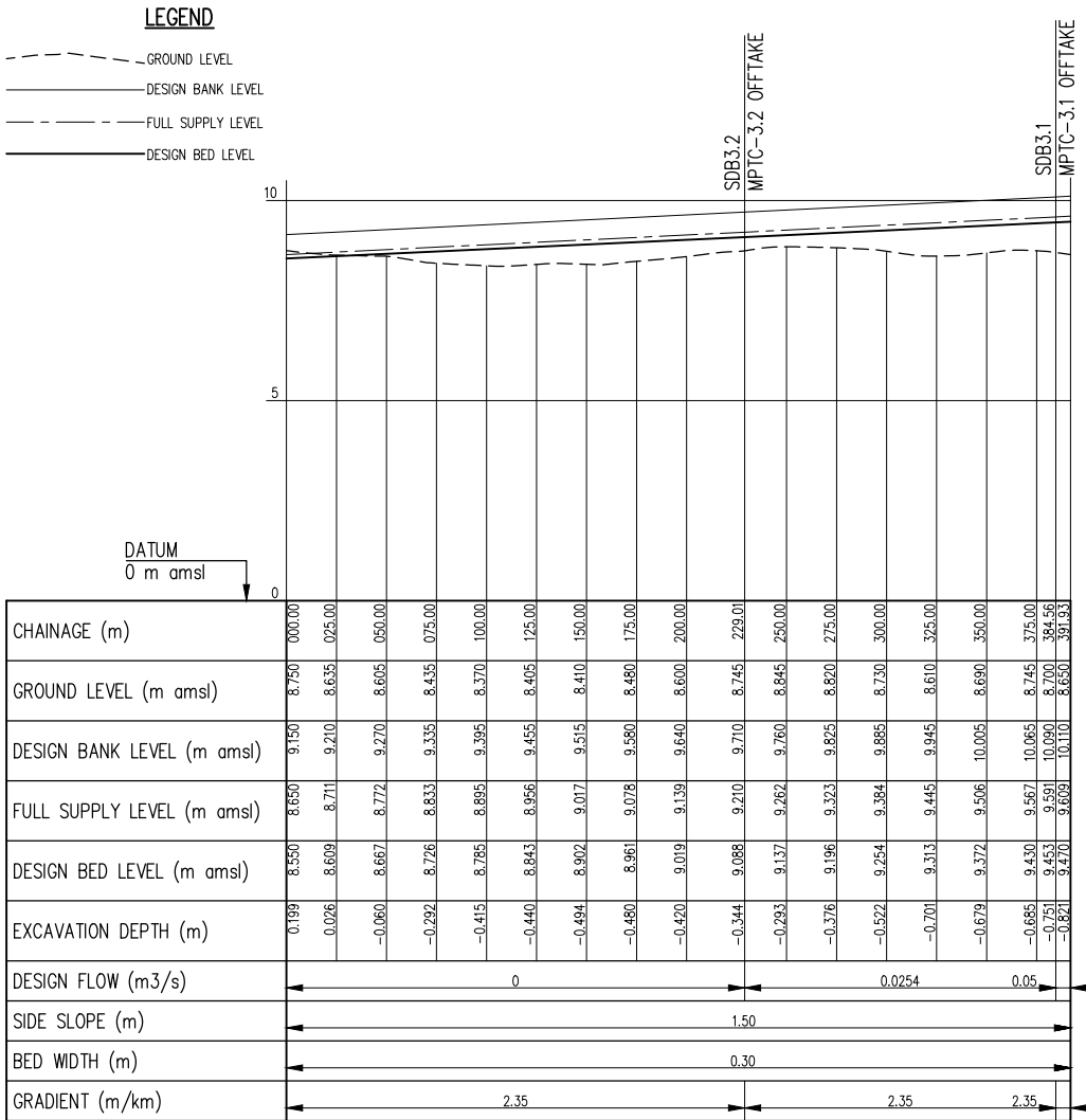
MPSC-3 PROFILE SCALE: Hor 1:2000, Ver 1:100
