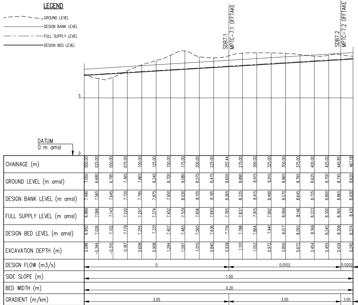
MPSC-7 PROFILE SCALE: Hor 1:2000, Ver 1:100
