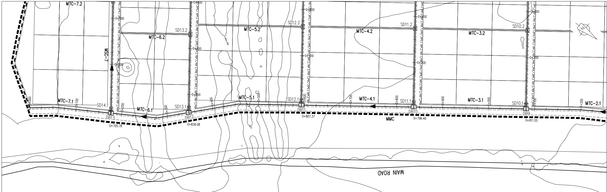
MMC / WMCC PLAN SCALE 1:2000
