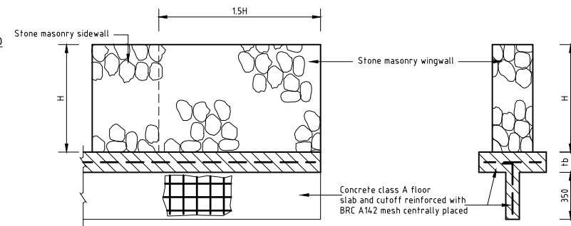
SECTION F-F 1:20 (AT A1)
